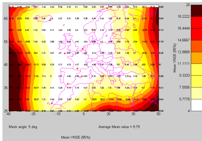
Fig. 9- Average VNSE of the ESTB
