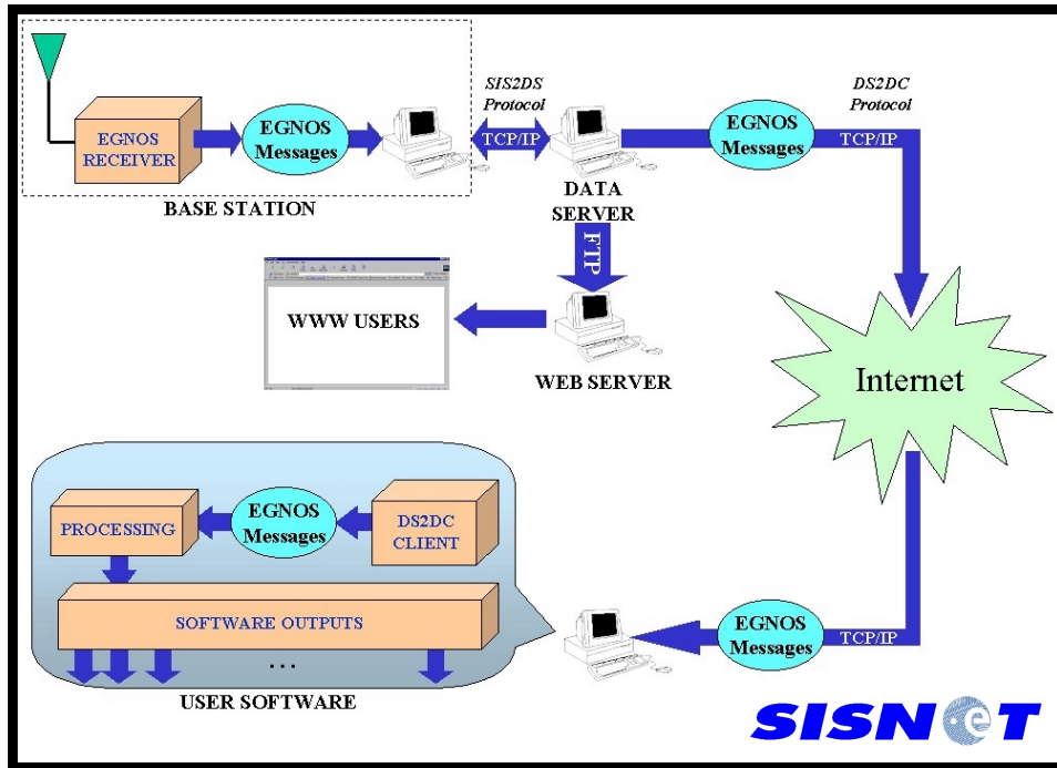
Fig. 6- Architecture of the SISNET platform
