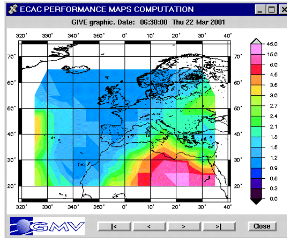
Fig. 5- GIVE estimates (ECUREV scenario, 9 RIMS)
