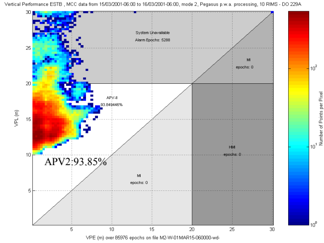
Fig. 7- VPL vs. VPE (24 hours duration)
