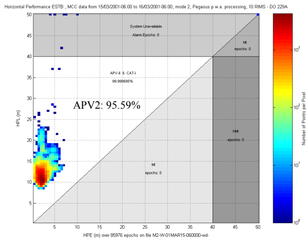
Fig. 8- HPL vs. HPE (24 hours duration)
